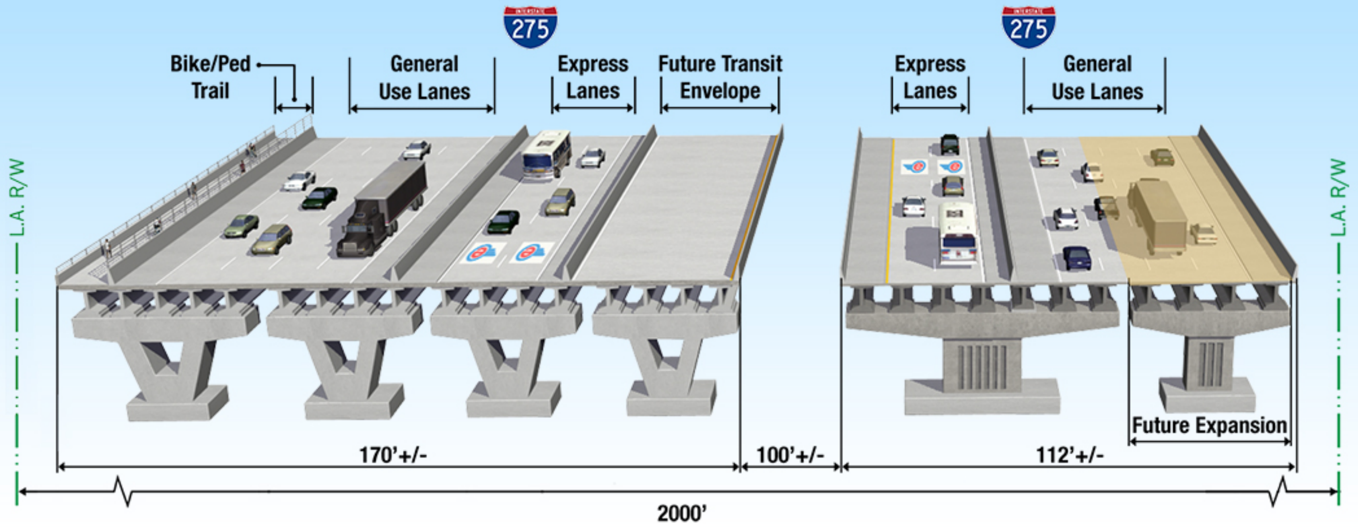
SOUTHBOUND BRIDGE WITH NORTHBOUND EXPRESS LANES CONVERTED TO TRANSIT ENVELOPE
